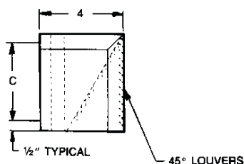
Figure 20: Fresh Air Intake Box Dimensions
