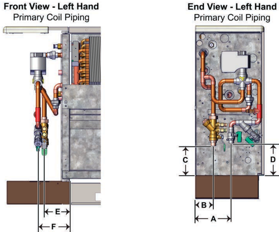
Figure 14: Hook Up Locations: 2-Pipe Arrangement
