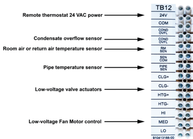
Figure 4: LV Terminal Strip 24 VAC connections
