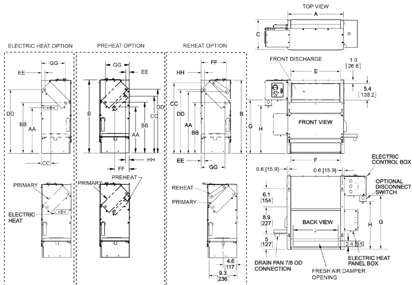
Figure 17: Dimensions: Hideaway, Front-Discharge Fan Coils
