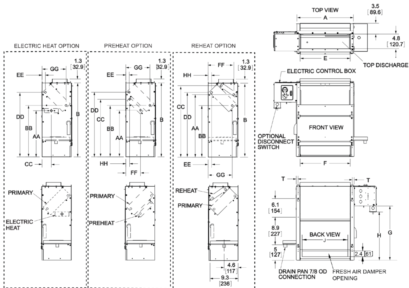
Figure 18: Dimensions: Hideaway, Top-Discharge Fan Coils
