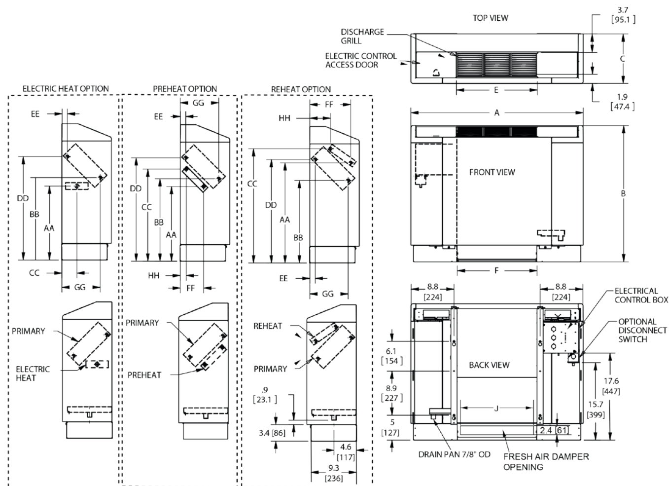
Figure 16: Dimensions: Slope Top Fan Coils
