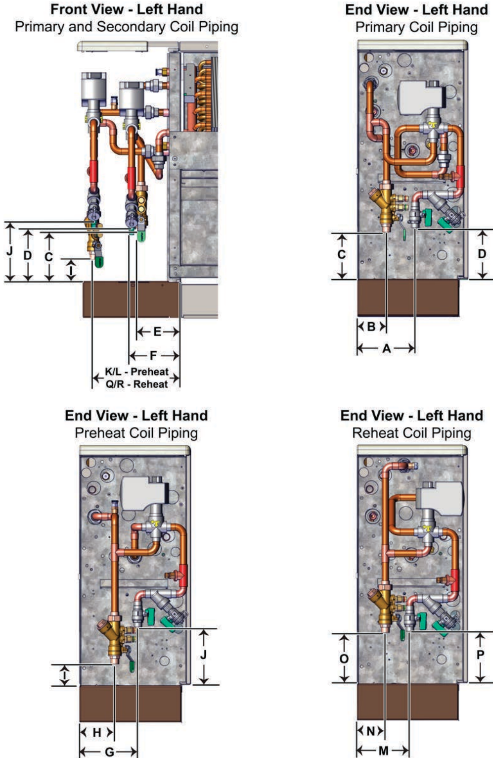
Figure 12: Hook Up Locations: 4-Pipe Arrangement with Same-End Connections
