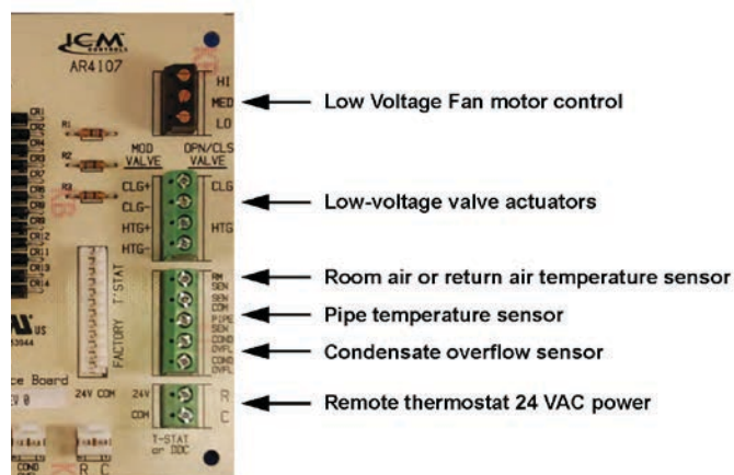
Figure 3: LV Interface Board 24 VAC connections
