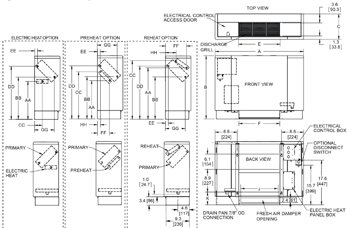
Figure 15: Dimensions: Flat Top Fan Coils
