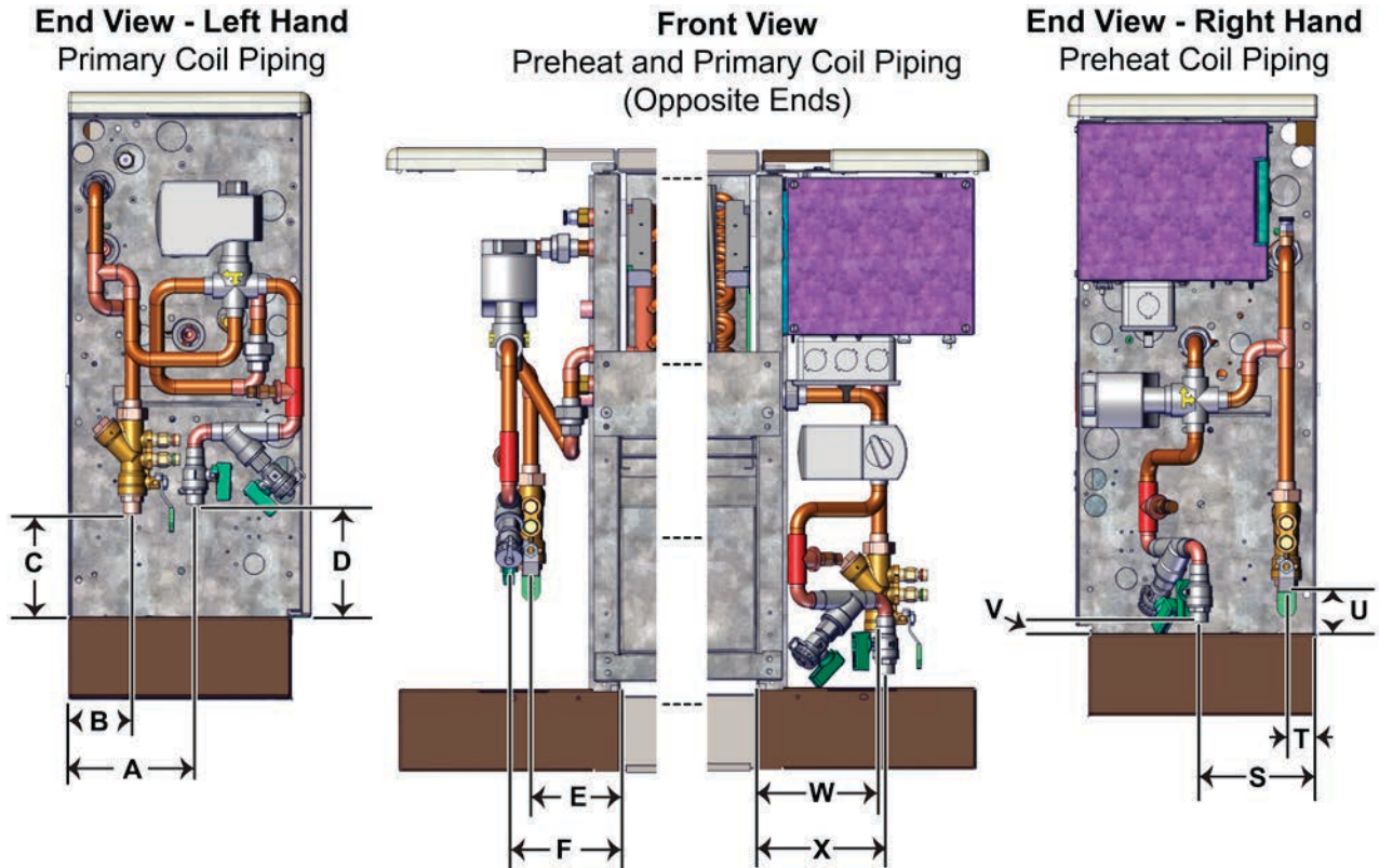
Figure 14: Hook Up Locations: 2-Pipe Arrangement
